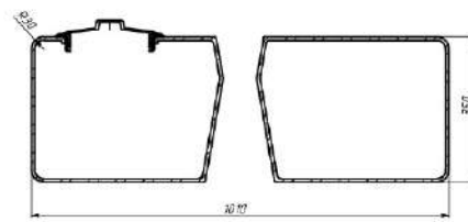
CROSS-SECTION B-B
