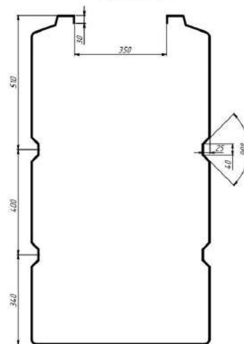
CROSS-SECTION A-A SCALE 1:5
